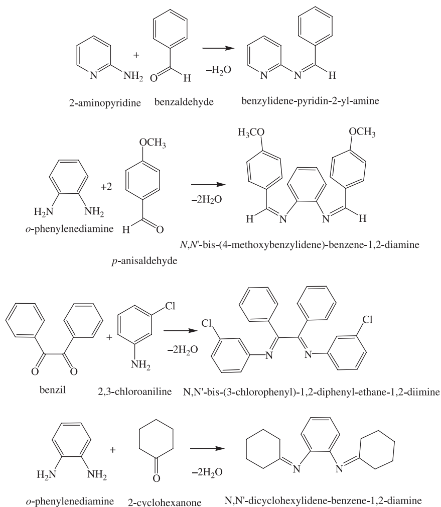
Scheme 1. Synthesis of ligands.
