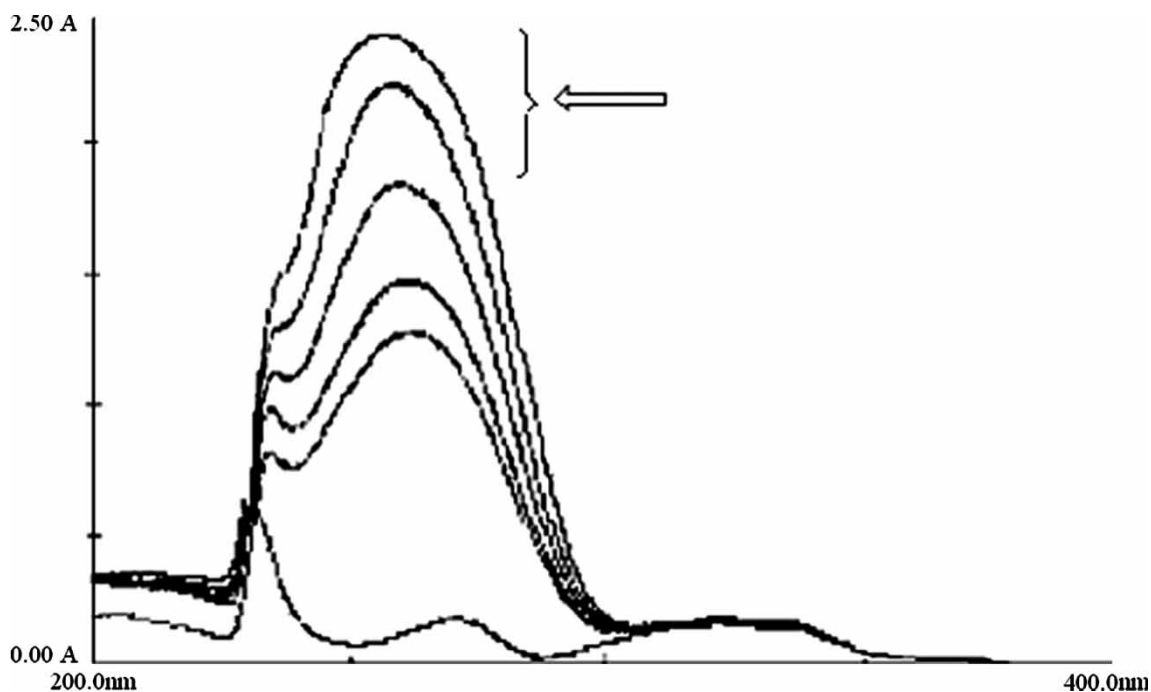
Figure 2. Absorption spectra of complex [\text{Fe}_2(\text{L})_2(\text{A}^1)_2(\text{pip})]\cdot 5\text{H}_2\text{O} in absence and presence of DNA.
