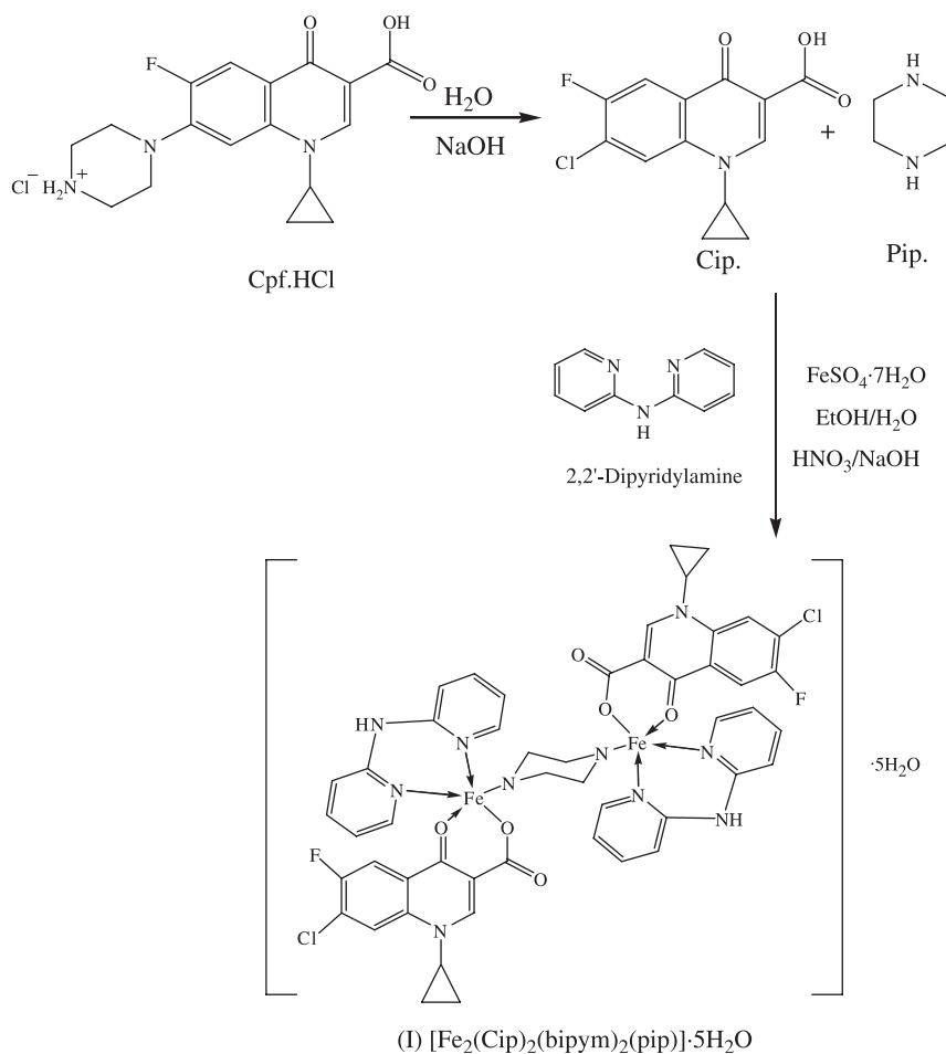
Scheme 2. Proposed reactions for the dimeric complex formation.
