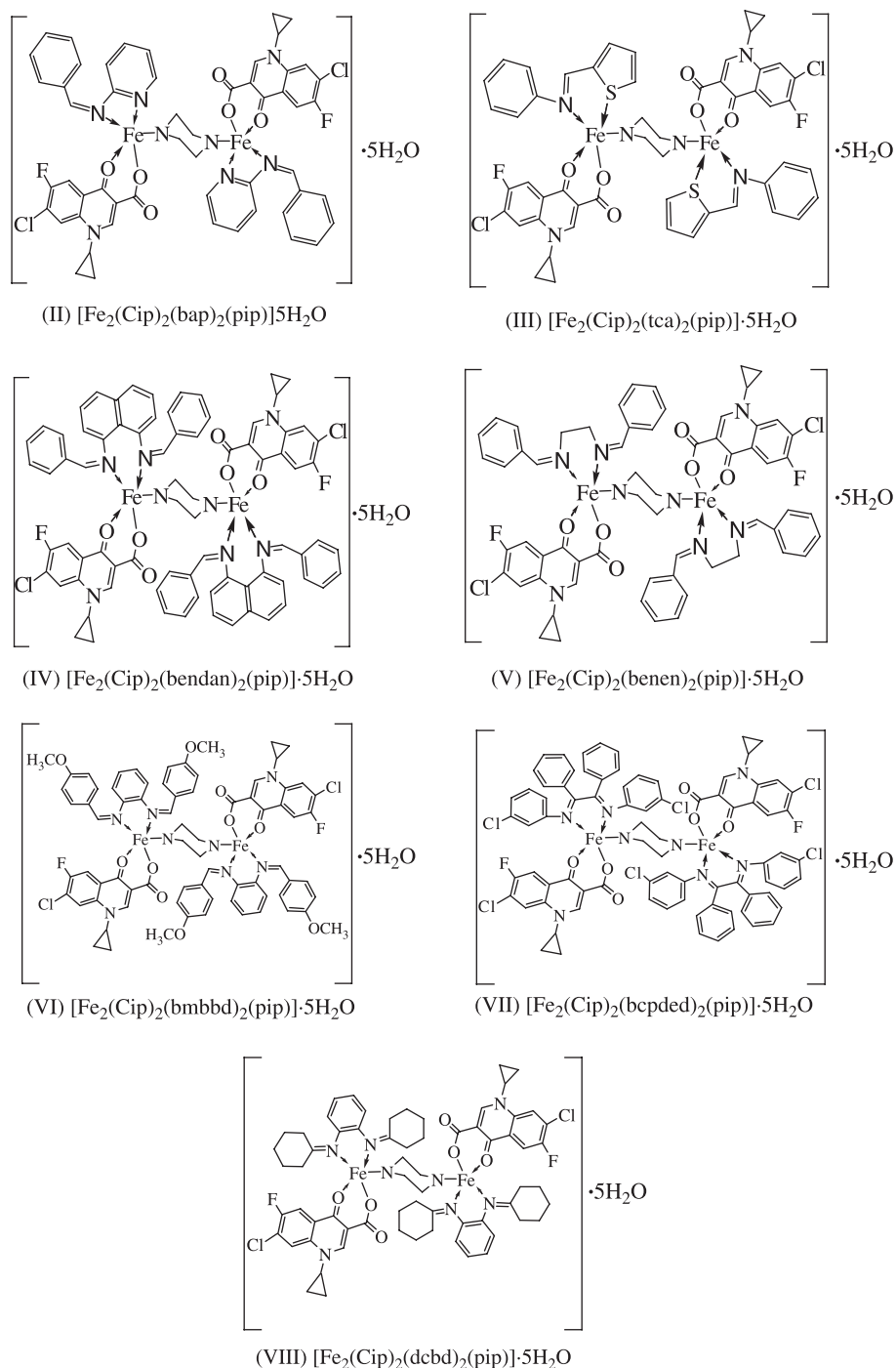
Figure 1. Suggested structures of the complexes.
